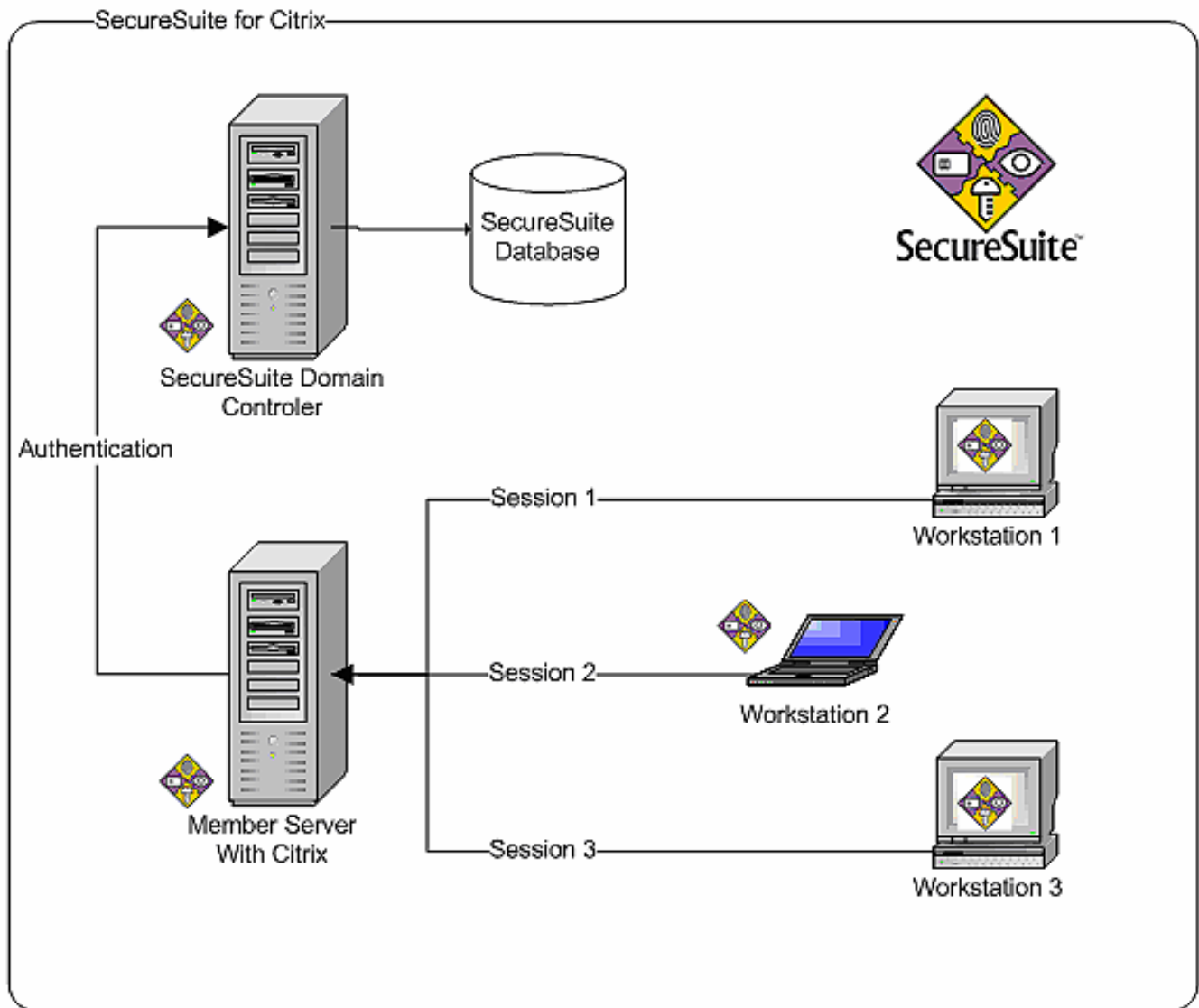
Diagram of SecureSuite-Citrix Architecture
